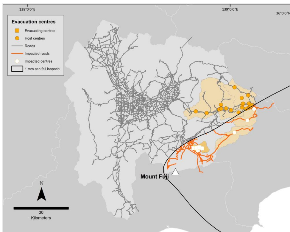
Figure 4.28: The exposure of roads and evacuation centres in Oshino, Otsuki, Uenohara and Doshi to 1 mm or more of ash fall from combined units. Impacted roads are in orange and isolated centres in white.
