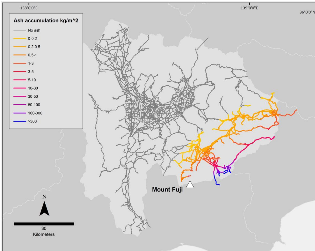
Figure 4.10: Exposure of roads to modelled ash fall accumulation loads ( \text{kg}/\text{m}^2 ) of the Hiei eruption using data from Magill et al. (2015). Cooler colours indicating higher ash loads.
