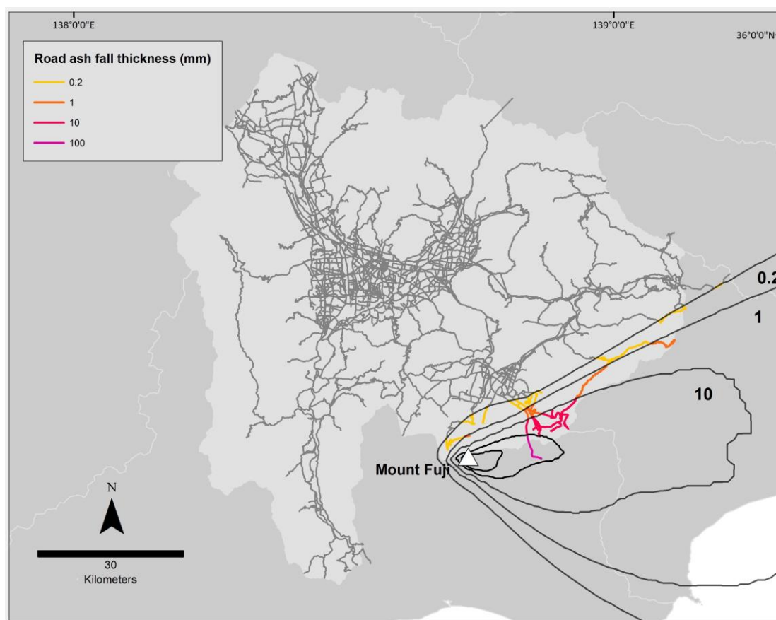
Figure 4.13: Exposure of prefecture roads to ash fall from unit A. Isopachs outlined in black and roads coloured with ash fall depths (mm). Note the inner isopachs represent 100 and 300 mm.
