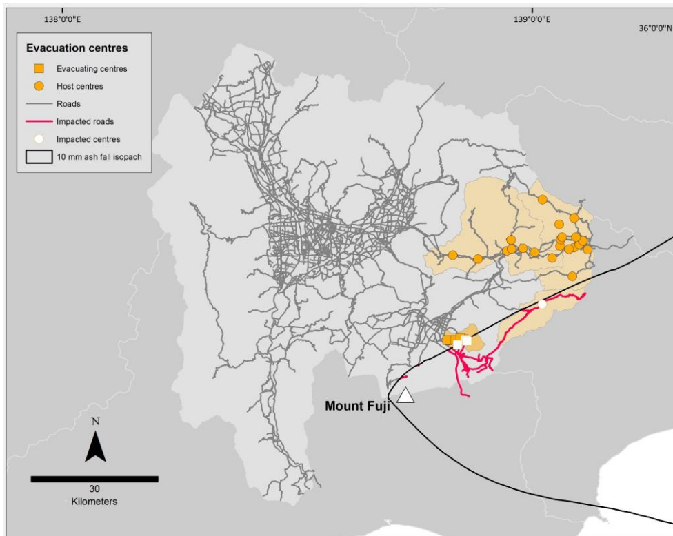
Figure 4.29: The exposure of roads and evacuation centres in Oshino, Otsuki, Uenohara and Doshi to 10 mm or more of ash fall from combined units. Impacted roads are in red and isolated centres in white.
