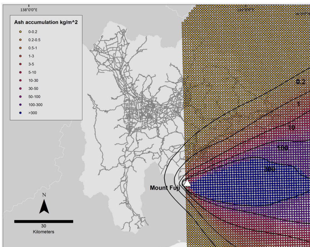
Figure 4.9: Simulated gridded ash fall accumulation load ( \text{kg}/\text{m}^2 ) and isopachs of the Hiei eruption modelled by Magill et al. (2015) overlaid onto Yamanashi Prefecture roads.
