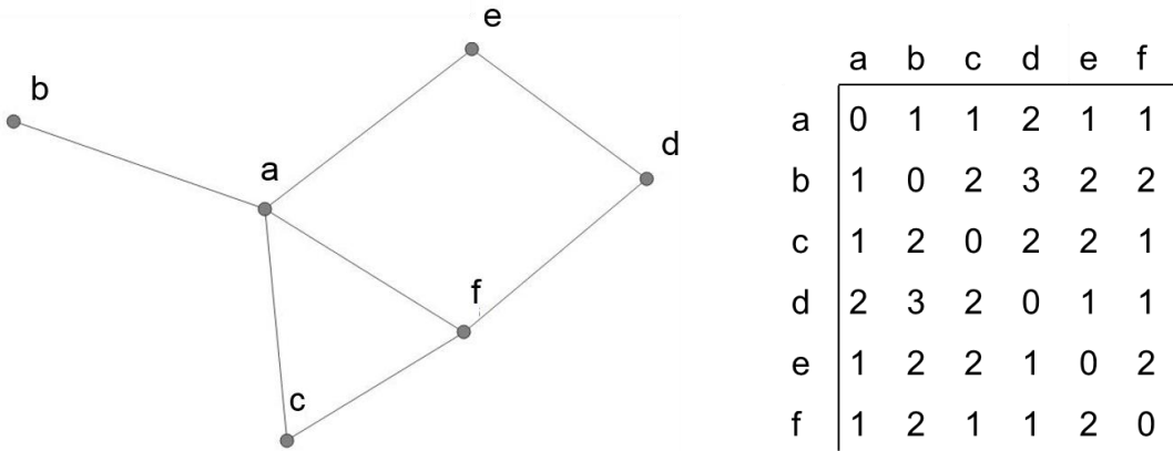
Figure 3.6: Geographical (left) and distance matrix (right) representations of example graph, with edge weight equal to 1.
