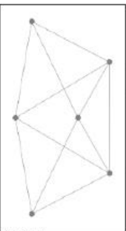
Fig. 1. Example of a graph with nodes and edges.
