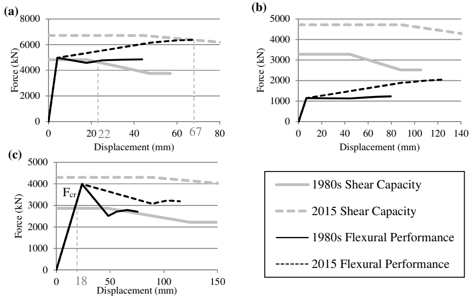
Figure 3 Displacement capacity of the individual C-shape wall for bending about the (a) major (b) minor (tension governing) and (c) minor (compression governing)
