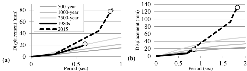
Figure 4 Displacement capacity of the buildings for bending about the (a) major axis and (b) minor axis and demand for different earthquake return periods
